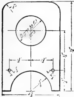
Fig. 4. Plan of front board which carries the objective
